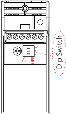
※ DALI interface(4 channels output, for DA2Q Model)
